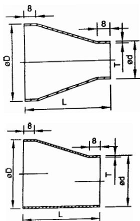
SMS Eccentric / Concentric Reducer
