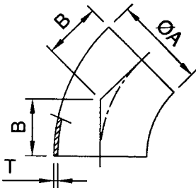
45° Short Elbow
