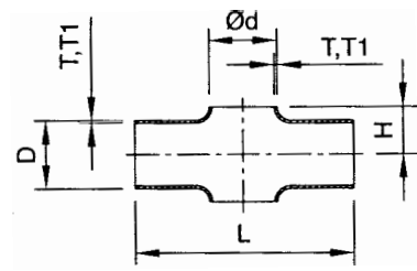
Welding Reducing Tee Without Straight-End
