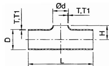
Welding Reducing Tee Without Straight-End
