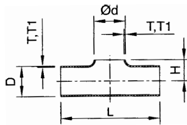
Tee Without Straight-End
