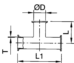
Clamp Tee
