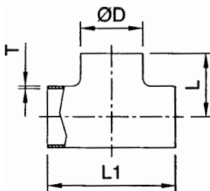
Welding Tee
