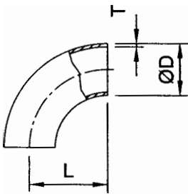
90° Short Bend
