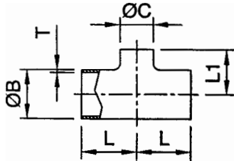
L7RW-Long Reducing Tee
