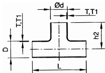
Tee With Straight-End
