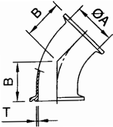
45° Clamp Elbow
