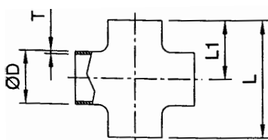
Cross
