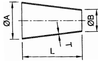
L31-Concentric Reducer
