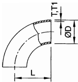
90° Tube Bend
