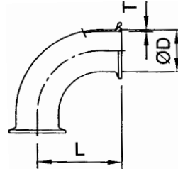
90° Clamp Bend
