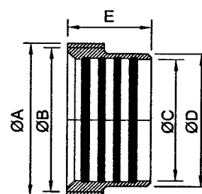
3A Recessless Male
