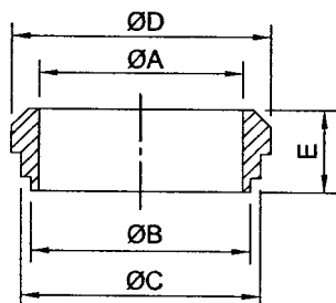
3A Short Bevel Seat Weld Liner 3A-14PRF
