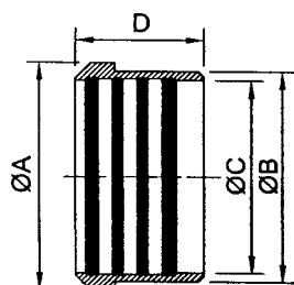
3A Recessless Liner
