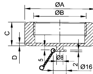
IDF-Blanks Nut IDF-13HBN
