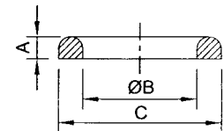
DIN Seal Ring (EPDM, Silicon, Viton)
