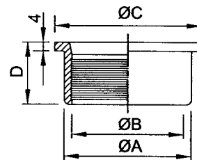
RJT Expanding Liner RJT-14R
