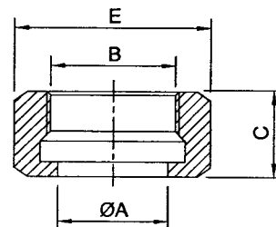
3A Hexagonal Nut 3A-13H
