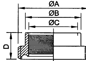
RJT Expanding Male RJT-15R
