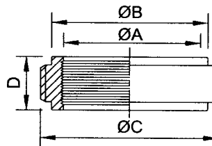
IDF Expanding Male IDF-15R
