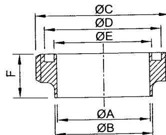
CL-Style Welding Male SMS-15G
