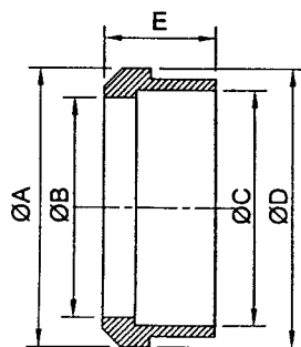
3A Recessless Liner
