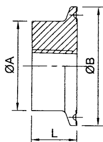
22MP Female Adapter
