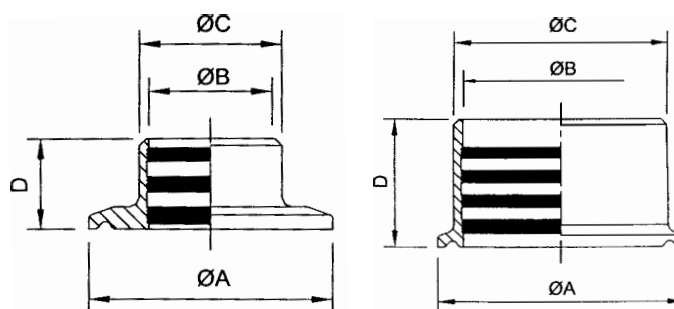
3A-Expanding Ferrule
