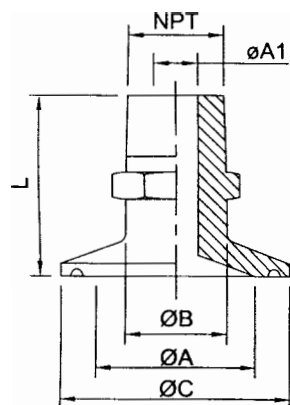
21MP Male Adapter
