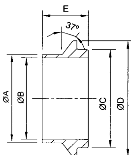
14WI I-LINE Ferrule
