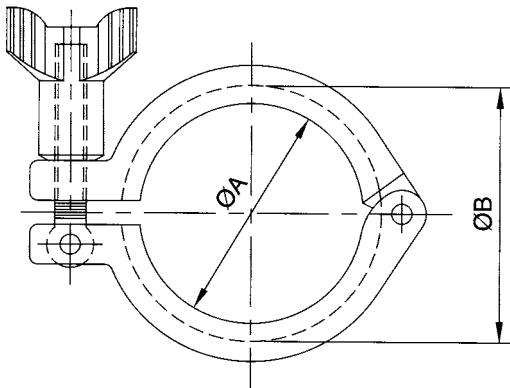
13MHH Heavy Duty Single Pin Clamp
