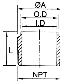
22MP Female Adapter
