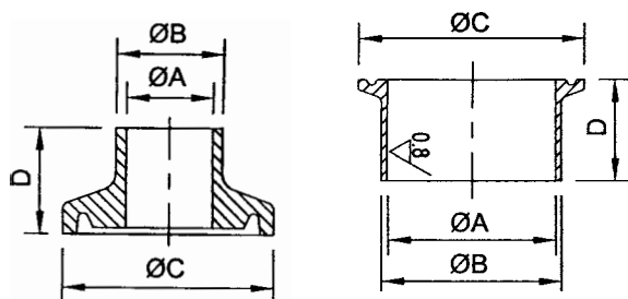
Welding Ferrule 3A/SMS-14WMP 14MMP 14AMP
